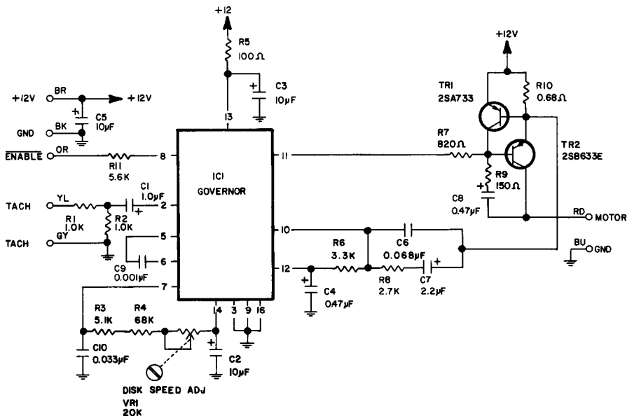
Fig. 7-49. Schematic of drive motor servo circuit, Model 1542.
